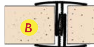
B as connecting profile for 16 or 19 mm panels
