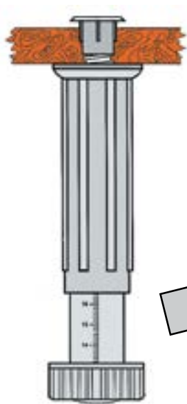
Furniture foot with dowel drilling ø 13 mm (dowel provided)
